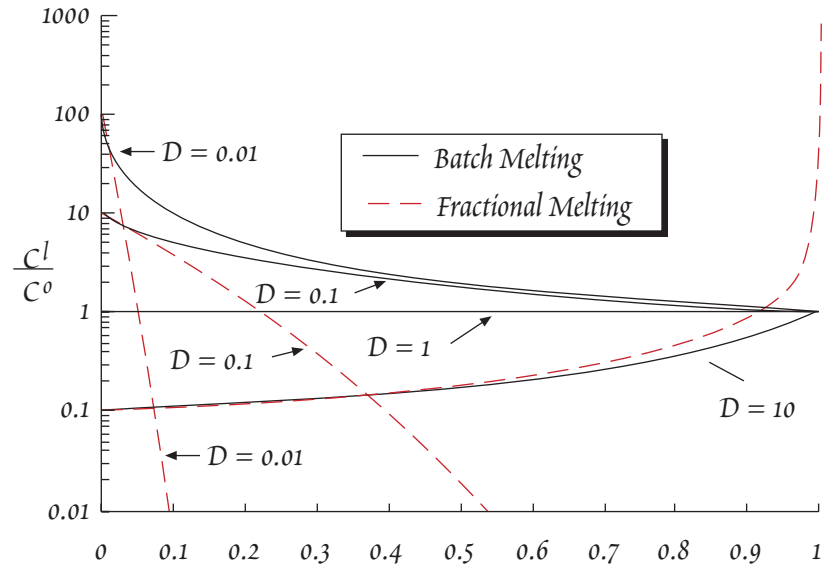
Figure 7.21. Variation in C^l/C^0 with degree of melting, F, for various partition coefficients for batch and fractional melting.
