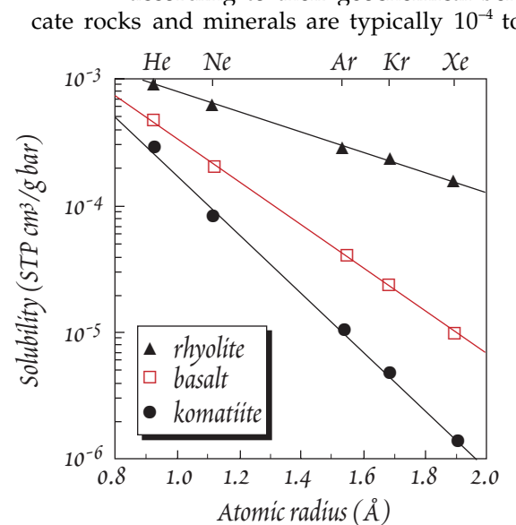
Figure 7.4. Solubility of the rare gases in melts of varying composition at 1200^\circ to 1400^\circ C. Solubility is a strong function of atomic radius and melt composition, but only a weak function of temperature. From Carroll and Draper (1994).
