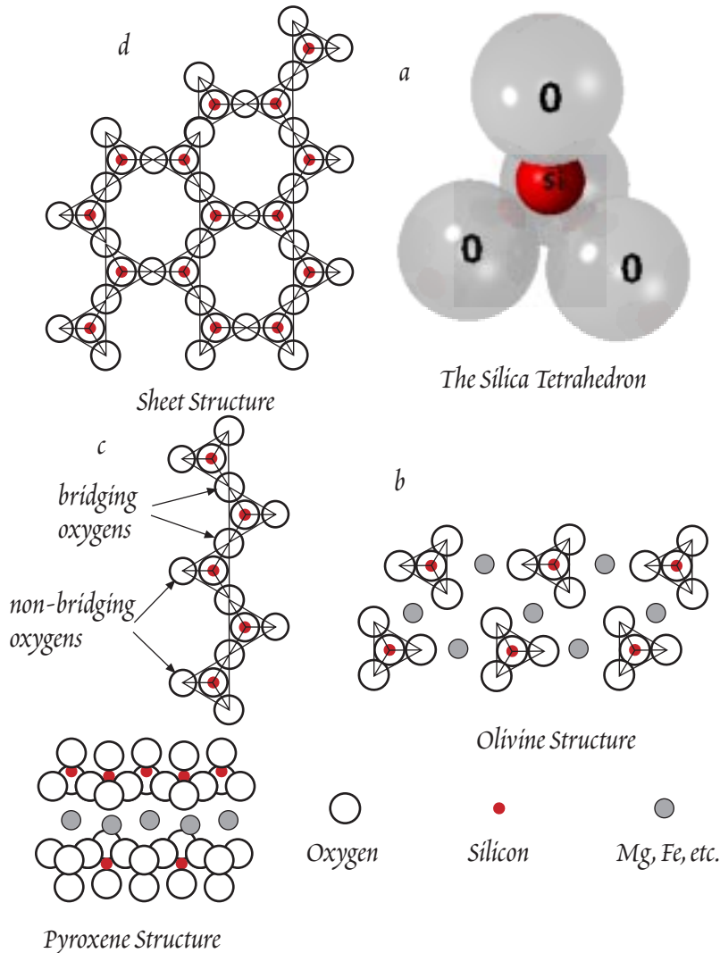
Figure 1.11. The silica tetrahedron and the structure of silicate minerals. a. The silica tetrahedron consists of a central silicon atom bound to 4 oxygens. b. In orthosilicates such as olivine, the tetrahedra are separate and each oxygen is also bound to other metal ions that occupy interstitial sites between the tetrahedra. c. In pyroxenes, the tetrahedra each share one oxygen and are bound together into chains. Metal ions are located between the chains. d. In sheet silicates, such as talc, mica, and clays, the tetrahedra each share 3 oxygens and are bound together into sheets.
