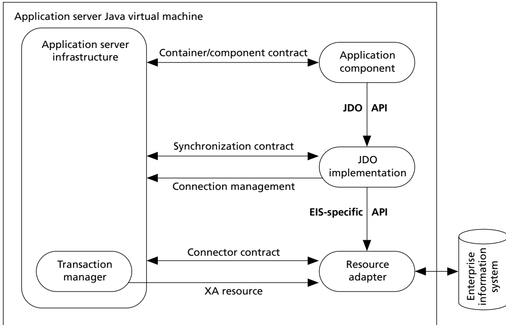
Figure 3.2 Managed environment
