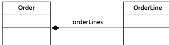
Figure 5.2 Order composition of OrderLine
