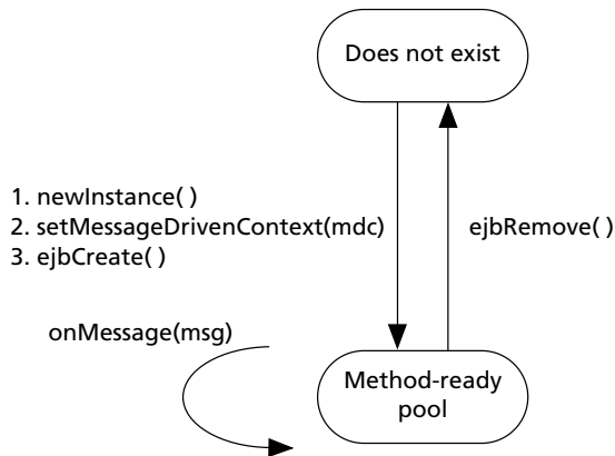
Figure 11.4 Message-driven bean lifecycle
