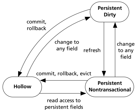
Figure 4.10 Optimistic transactions
