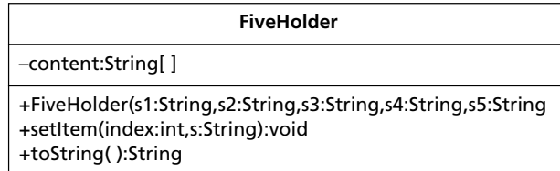
Figure 5.13 UML for FiveHolder
