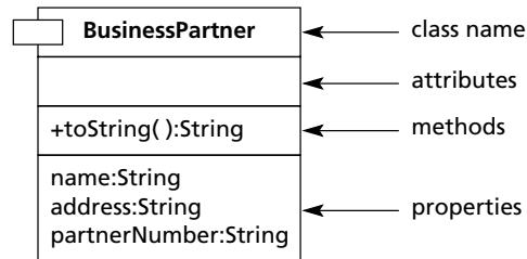
Figure 2.1 UML representation of BusinessPartner
