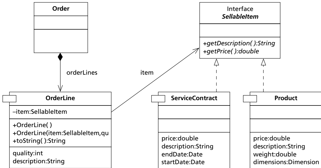
Figure 5.12 UML expanded
