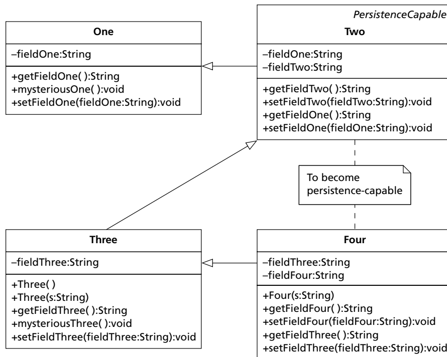
Figure 5.16 Completed inheritance hierarchy
