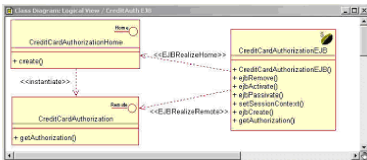
Figure 7: A stateless Session Bean
