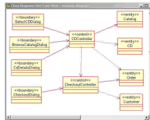
Figure 4: Preliminary analysis level class diagram
