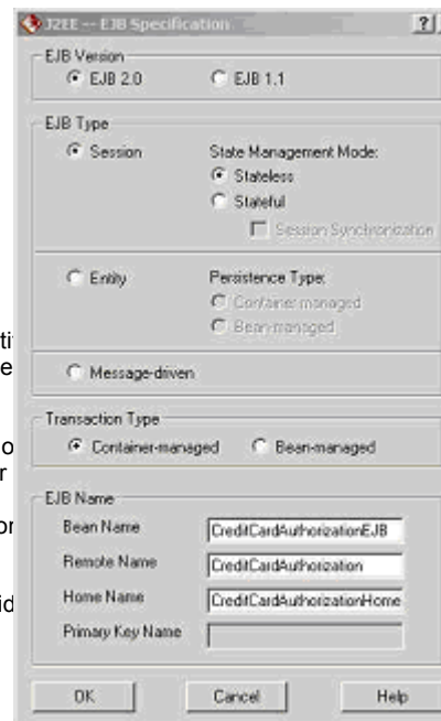
Figure 6: Creating an EJB Session Bean
