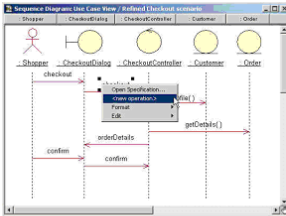
Figure 3: Refined sequence diagram with analysis objects
