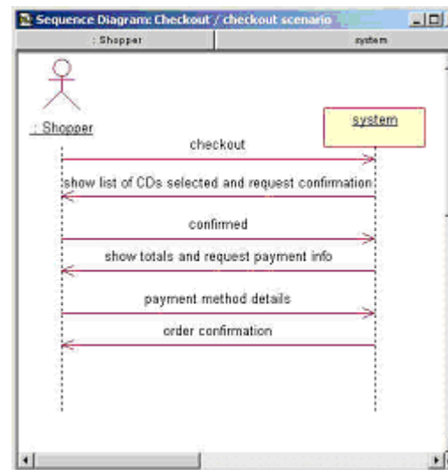
Figure 2: A sequence diagram illustrating checkout use case
