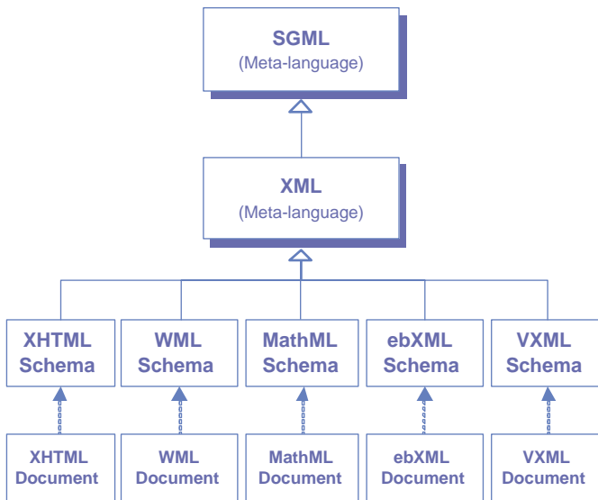
Figure 2.1 XML language hierarchy
