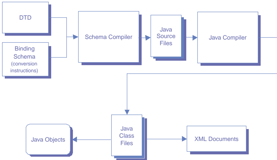
Figure 2.10 JAXB architecture
