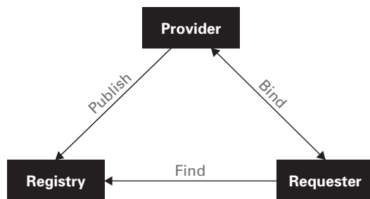
Figure 7.8 Web services loosen coupling between the provider and the requester by delaying the binding process. Providers publish their service in a distributed registry. Requesters can then search the registry for an appropriate service. When one is found, the service is bound between the requester and provider.
