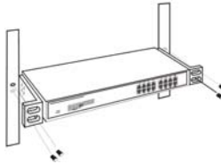
Figure 2. Mount the Switch in the rack
