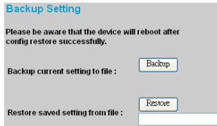
Figure 35. Backup Setting
