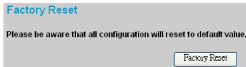
Figure 36. Reset Setting
