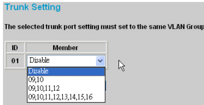
Figure 20. Trunk Settings
